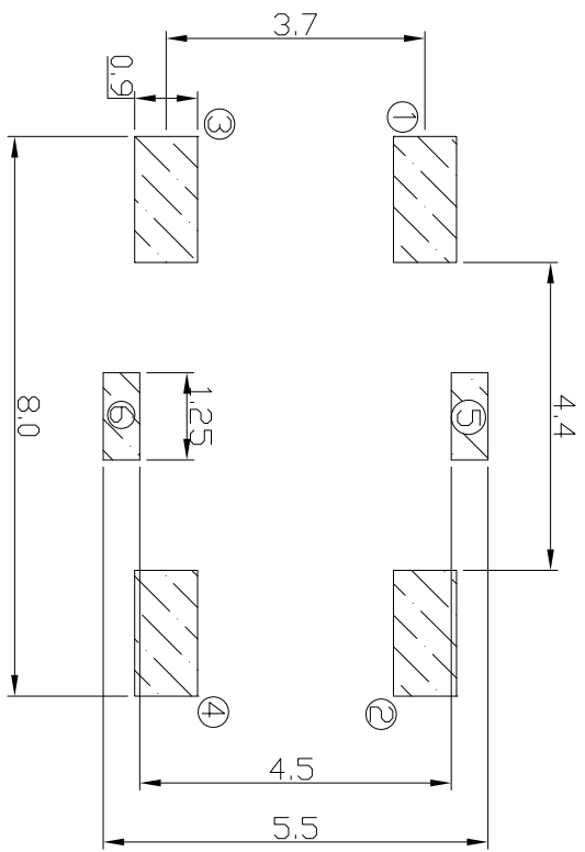
P. C. B LAYOUT
